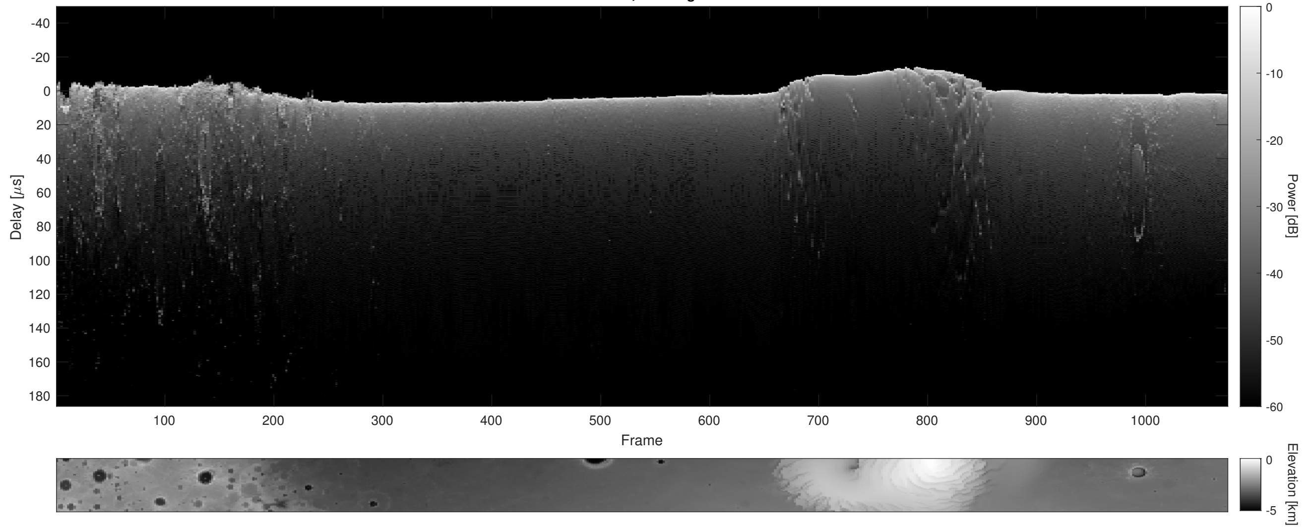
Orbit 7845, Cluttergram
