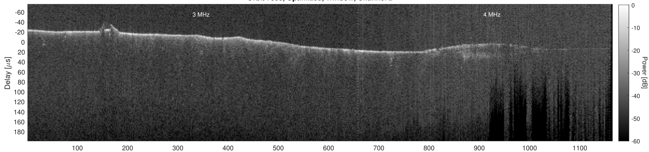
Orbit 7853, Cluttergram
