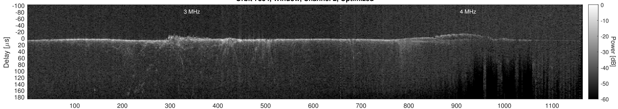
Orbit 7854, Cluttergram
