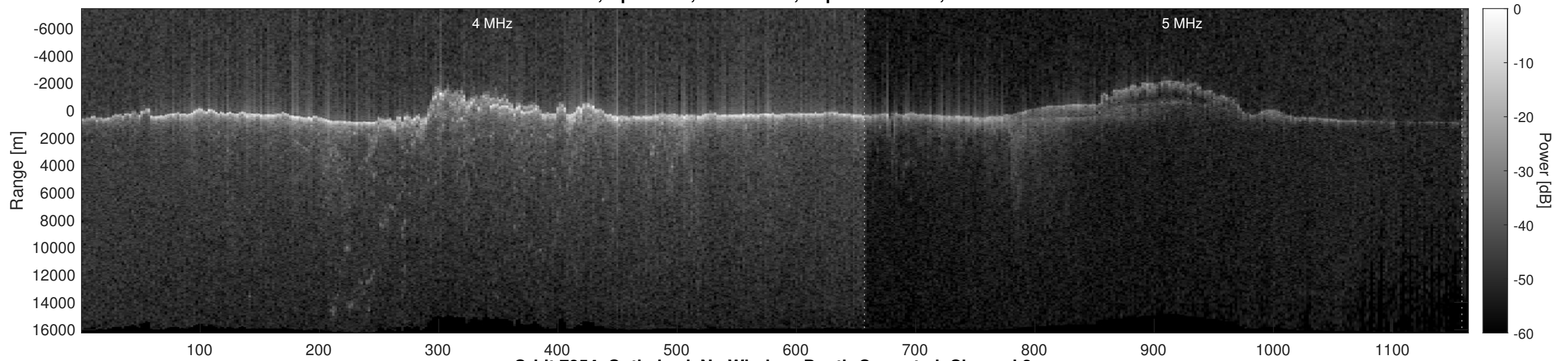
Orbit 7854, Optimized, No Window, Depth-Corrected, Channel 2
