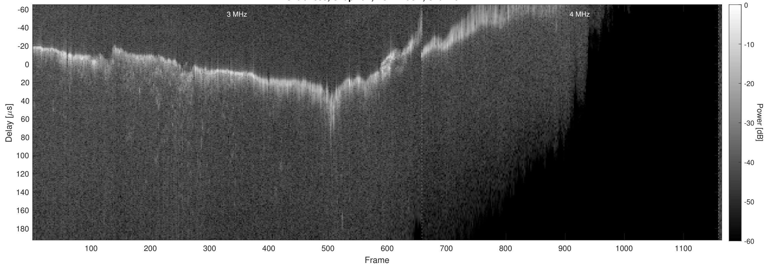
Orbit 7855, Chapman, No Window, Channel 2
