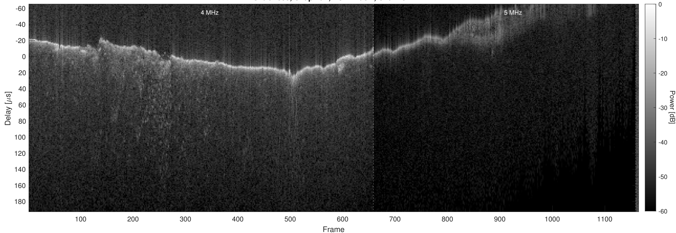
Orbit 7855, Chapman, No Window, Channel 2
