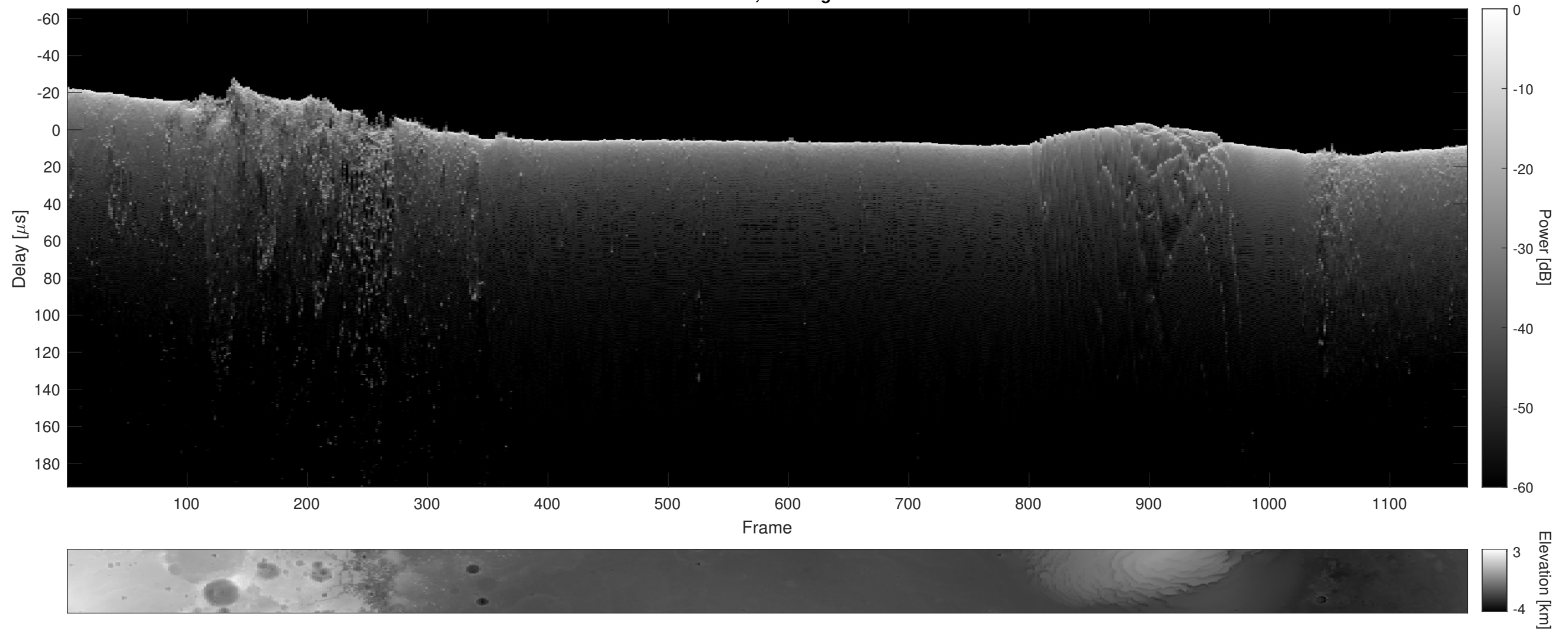
Orbit 7855, Cluttergram
