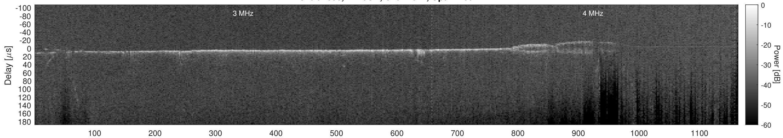
Orbit 7856, Cluttergram
