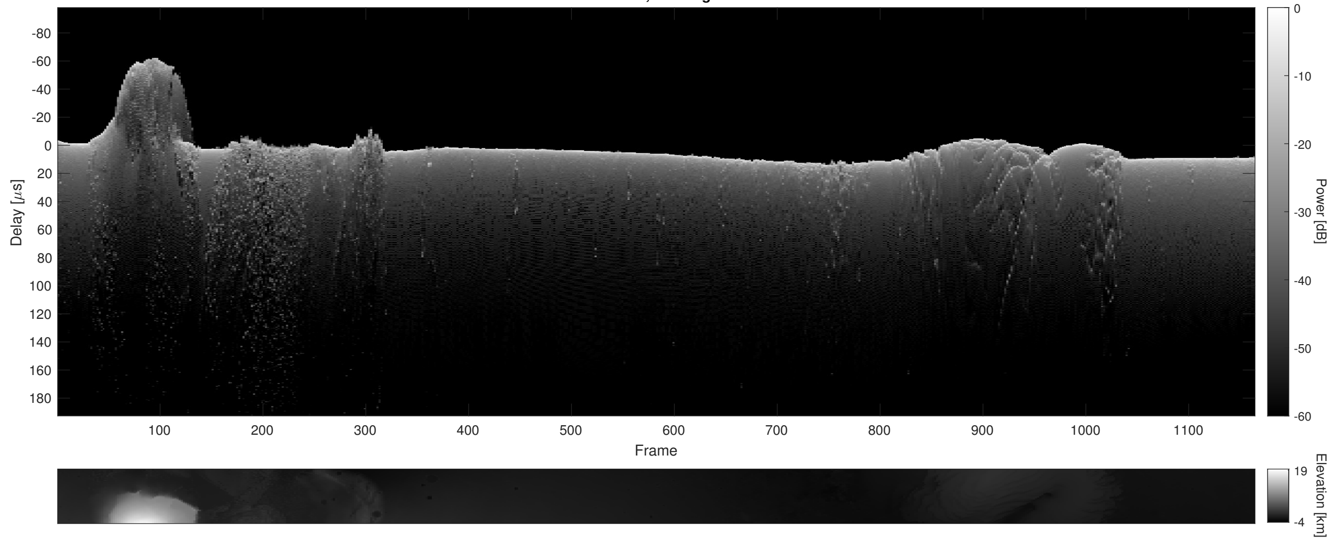
Orbit 7857, Cluttergram
