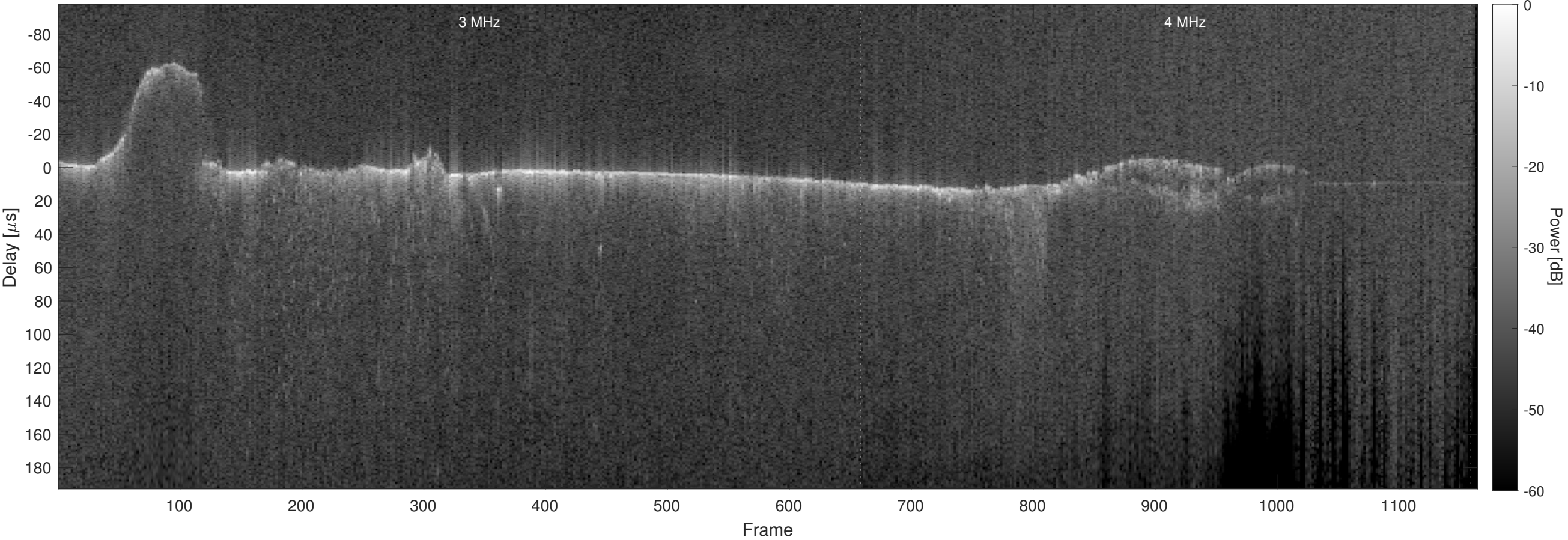
Orbit 7857, Optimized, No Window, Channel 2
