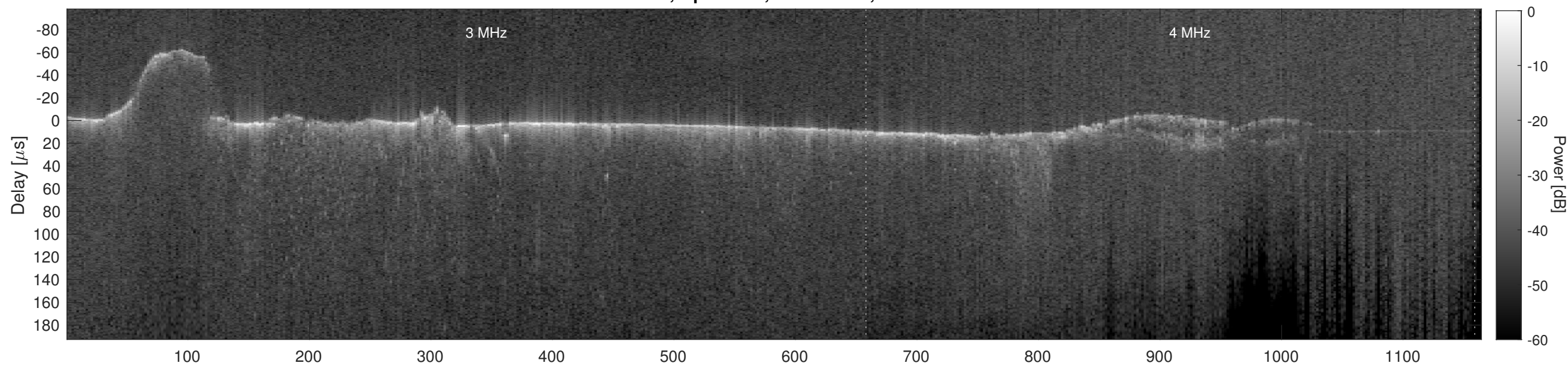
Orbit 7857, Cluttergram
