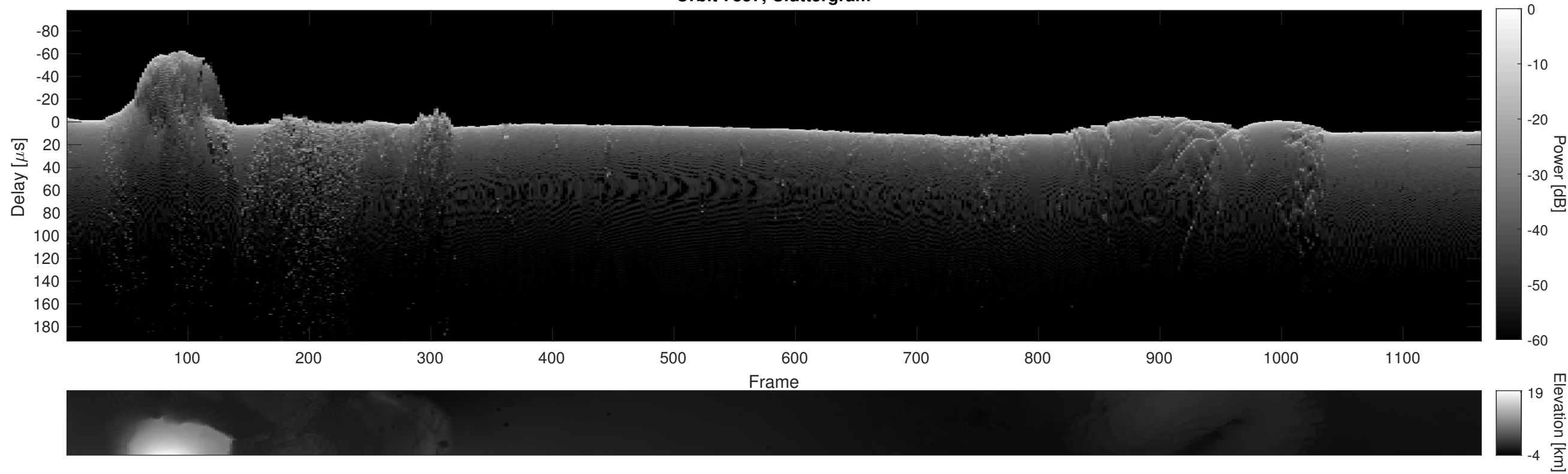
Orbit 7857, Cluttergram
