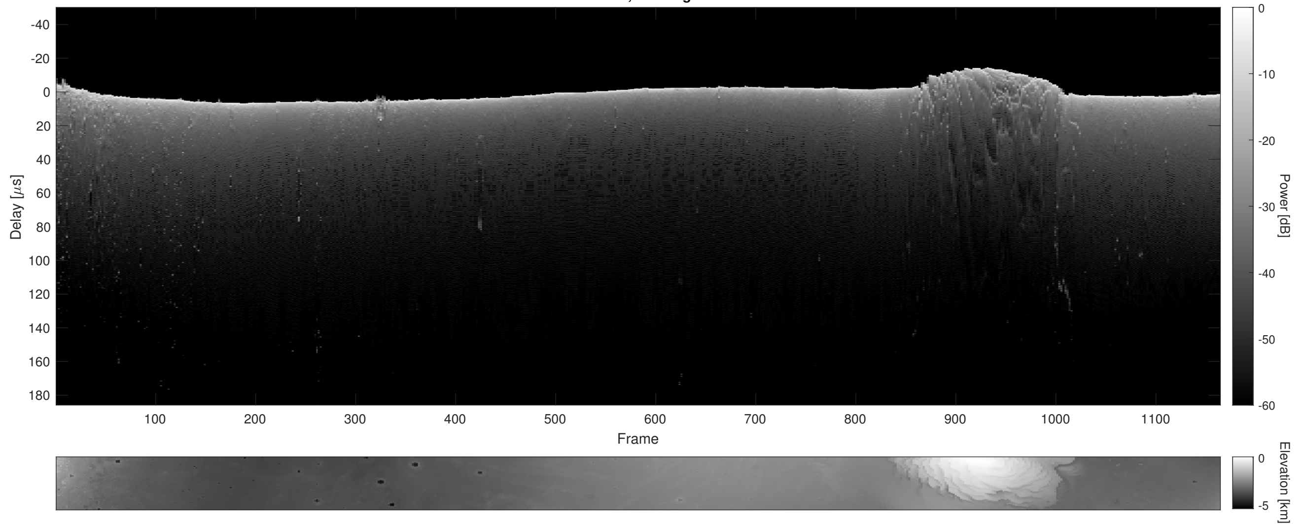
Orbit 7858, Cluttergram
