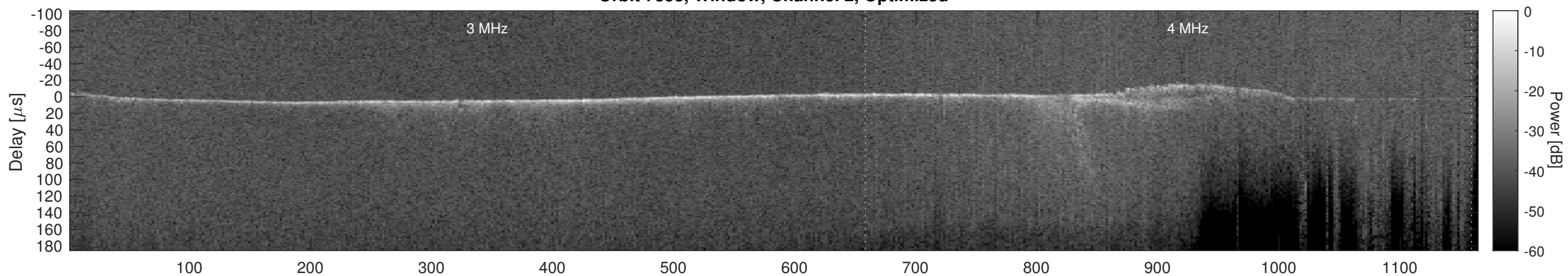
Orbit 7858, Cluttergram
