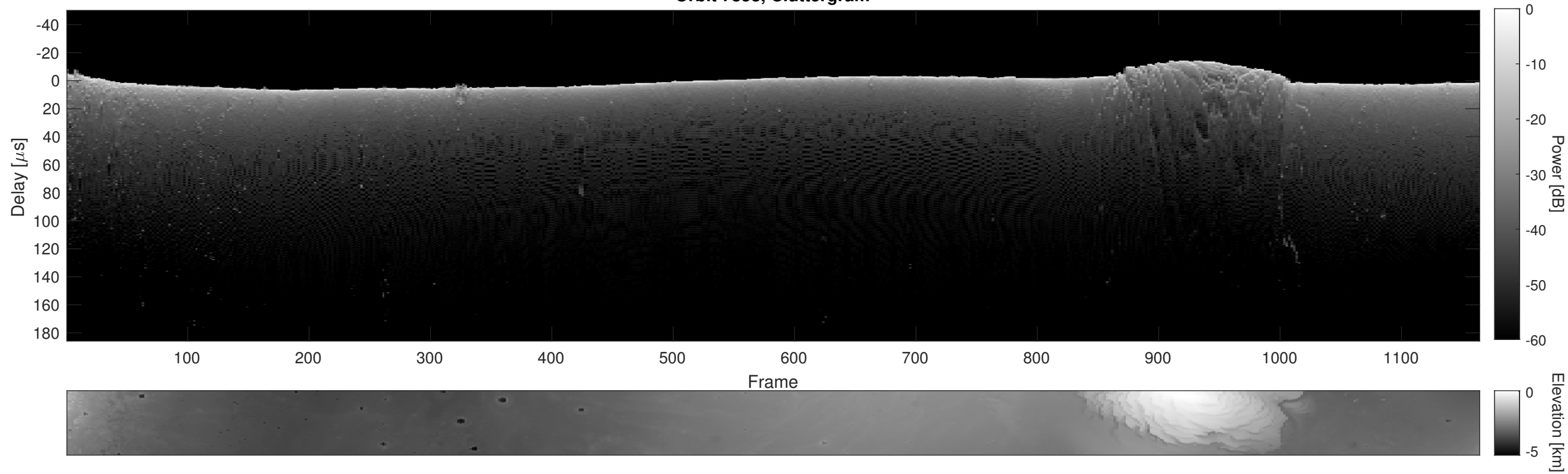
Orbit 7858, Cluttergram
