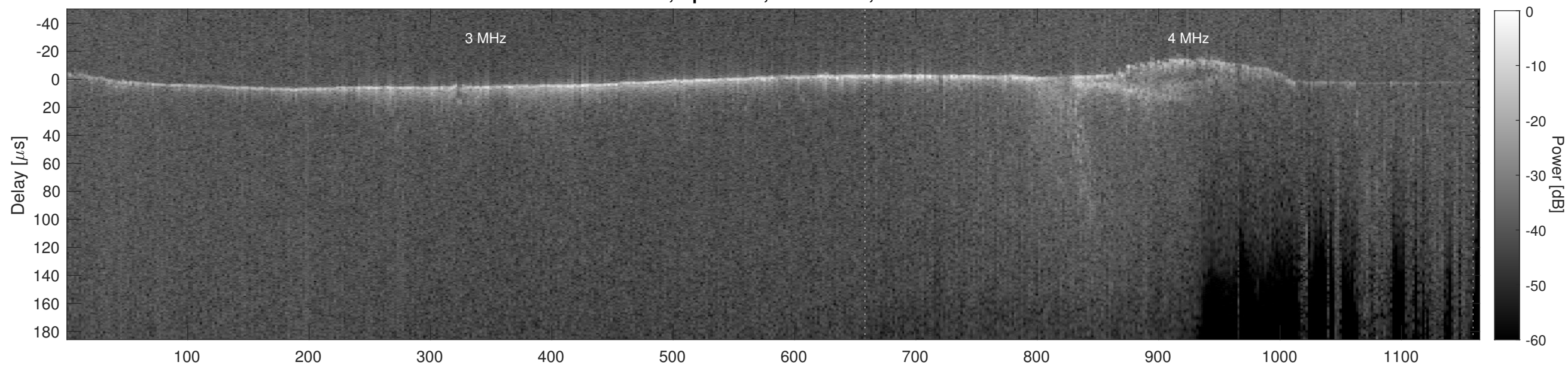
Orbit 7858, Cluttergram
