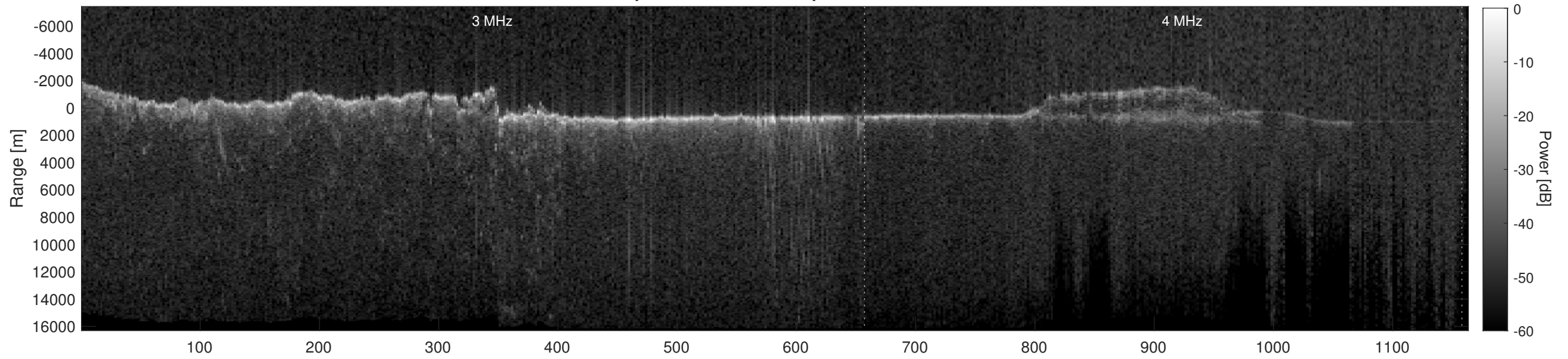
Orbit 7859, Depth-Corrected Cluttergram
