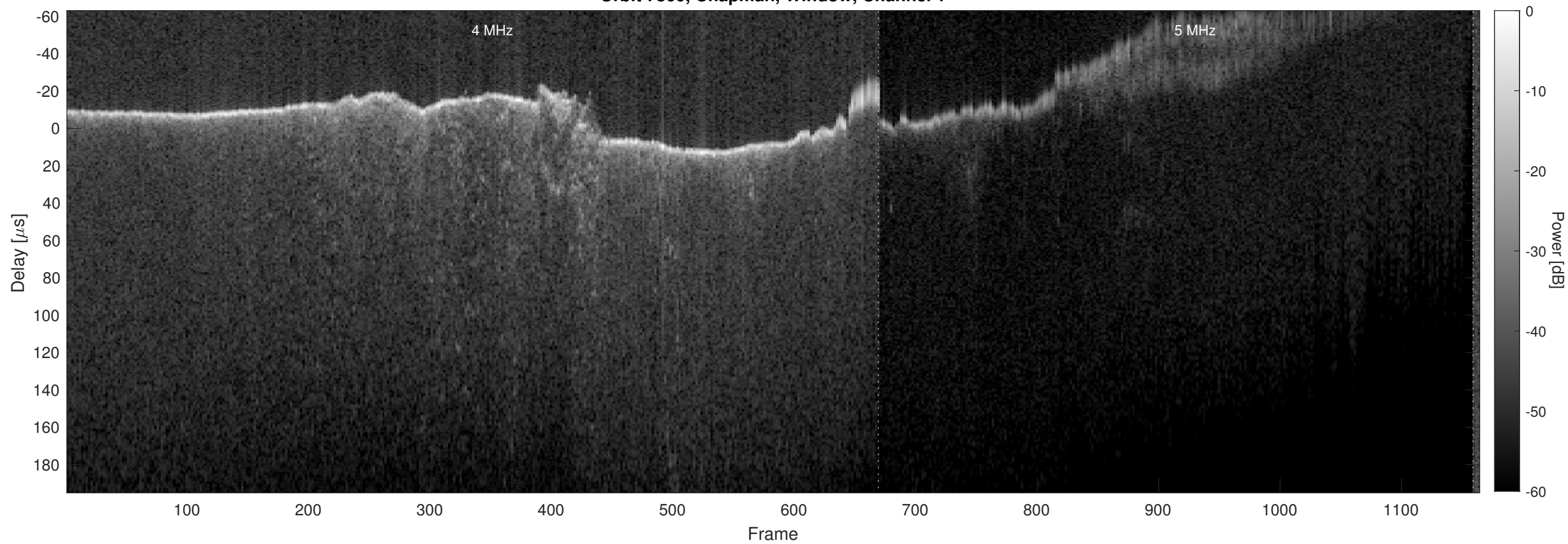
Orbit 7860, Chapman, Window, Channel 2
