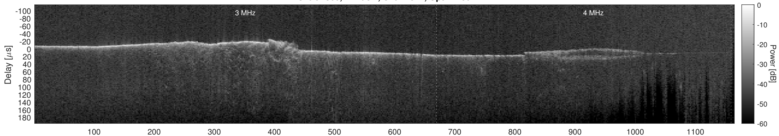
Orbit 7860, Cluttergram
