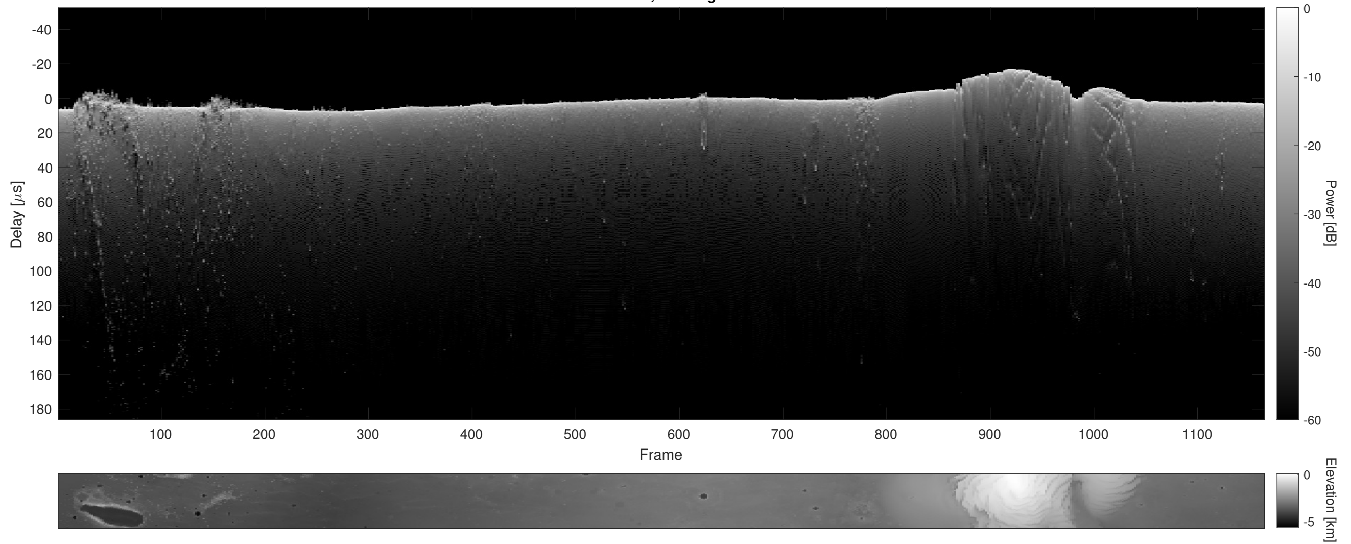
Orbit 7861, Cluttergram
