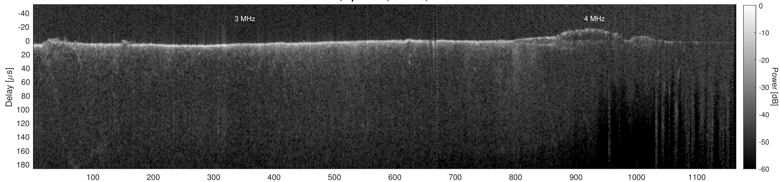
Orbit 7861, Cluttergram
