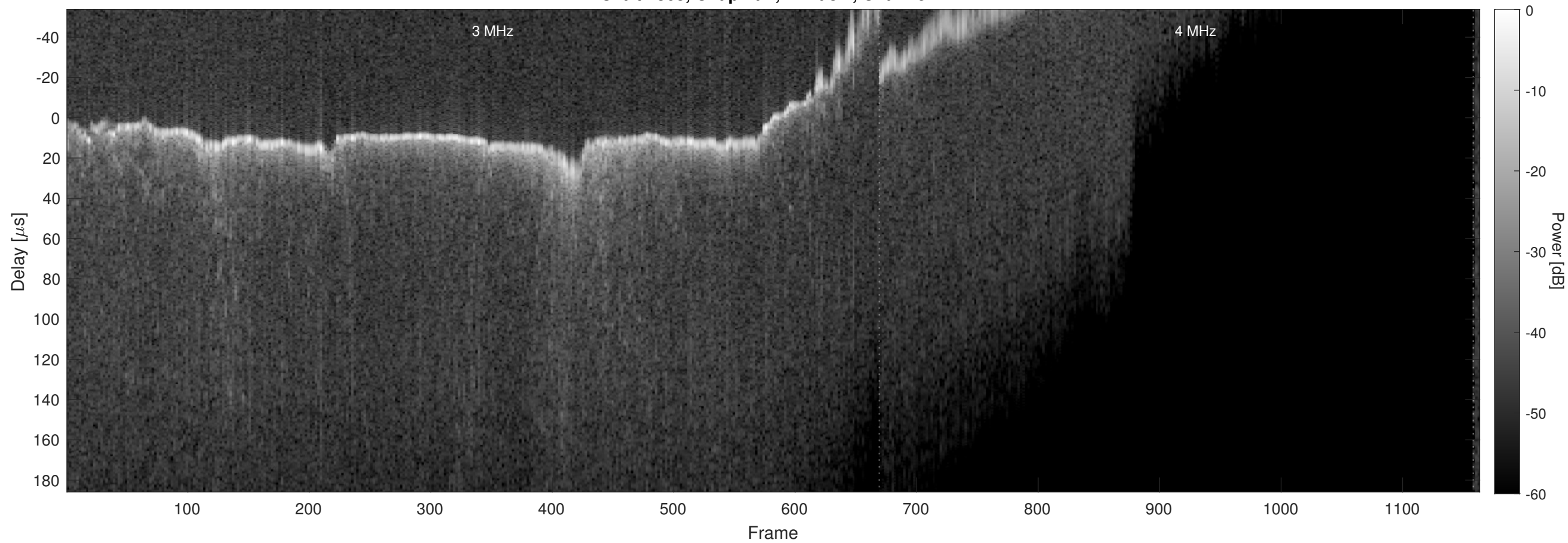
Orbit 7863, Chapman, Window, Channel 2
