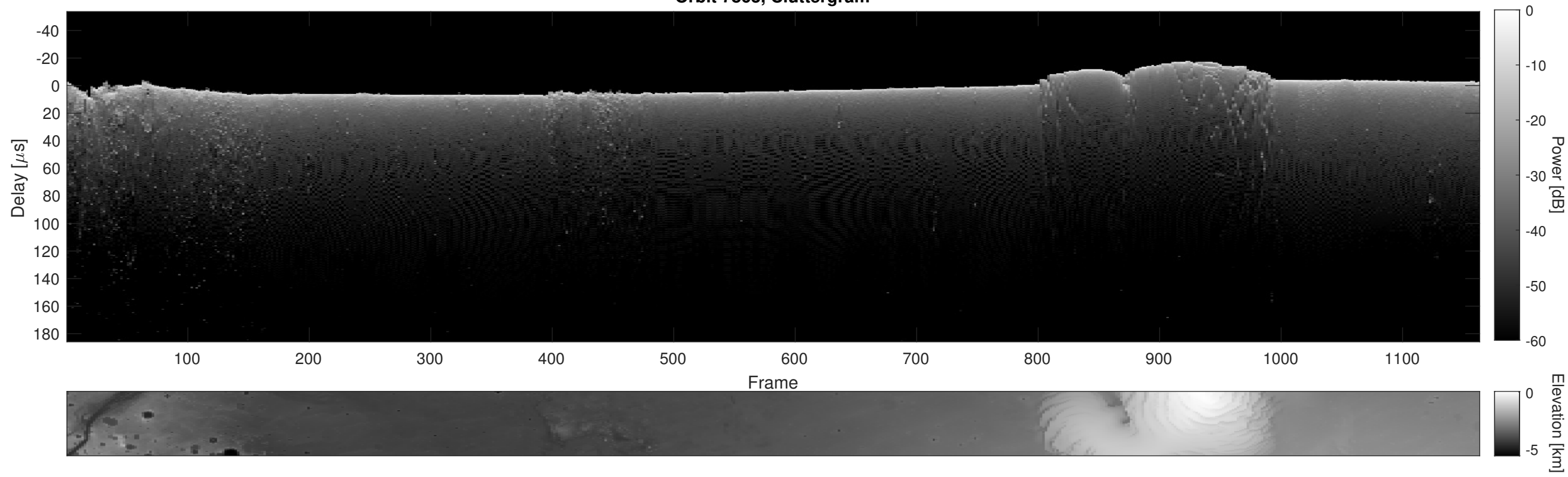
Orbit 7863, Cluttergram
