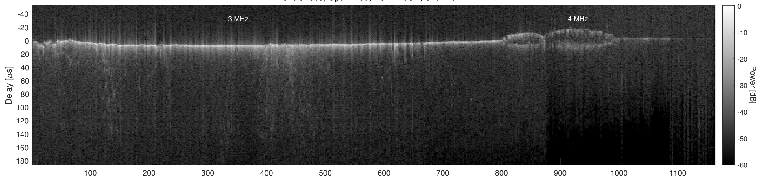
Orbit 7863, Cluttergram
