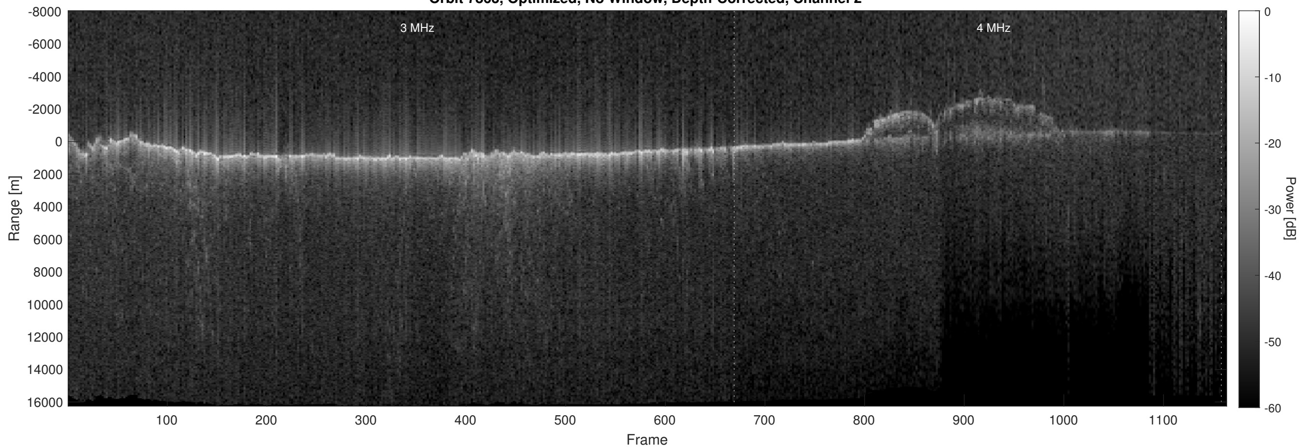
Orbit 7863, Optimized, No Window, Depth-Corrected, Channel 2
