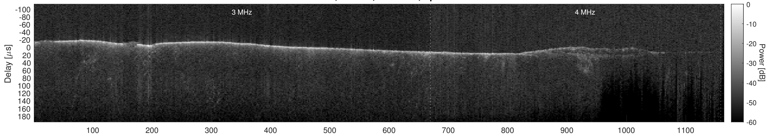
Orbit 7864, Cluttergram
