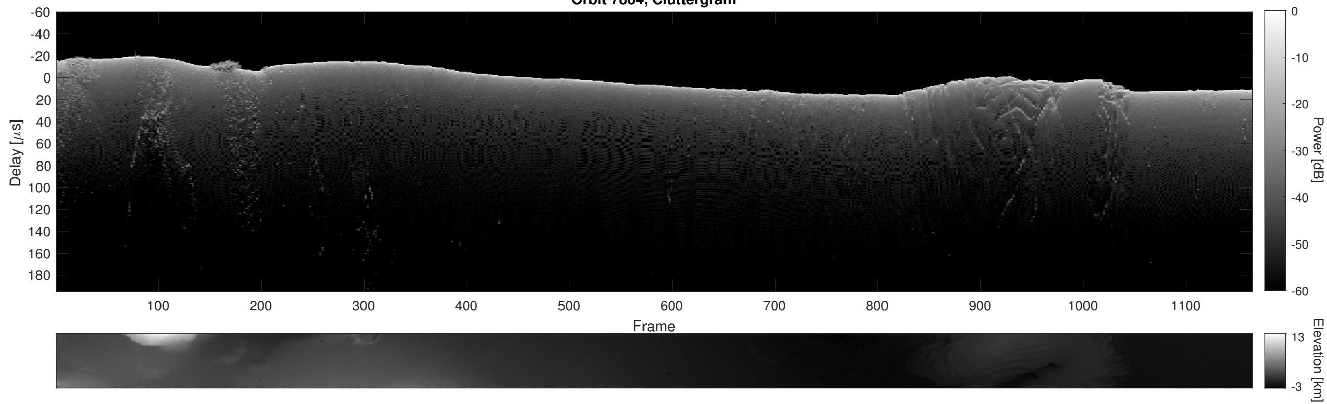
Orbit 7864, Cluttergram
