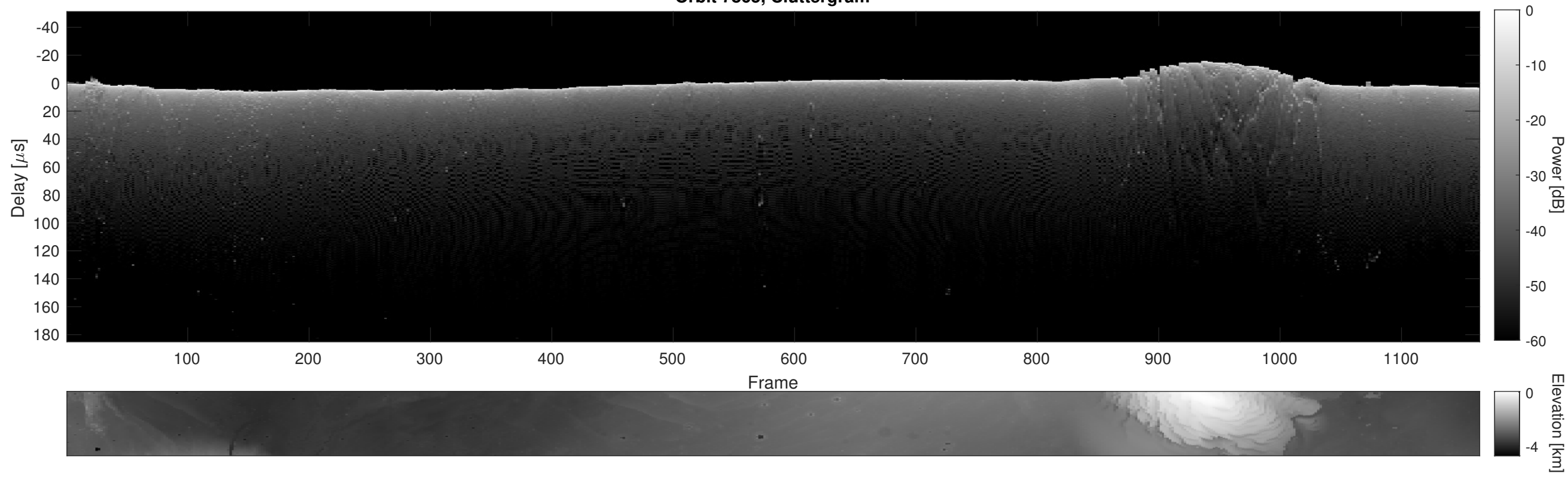
Orbit 7865, Cluttergram
