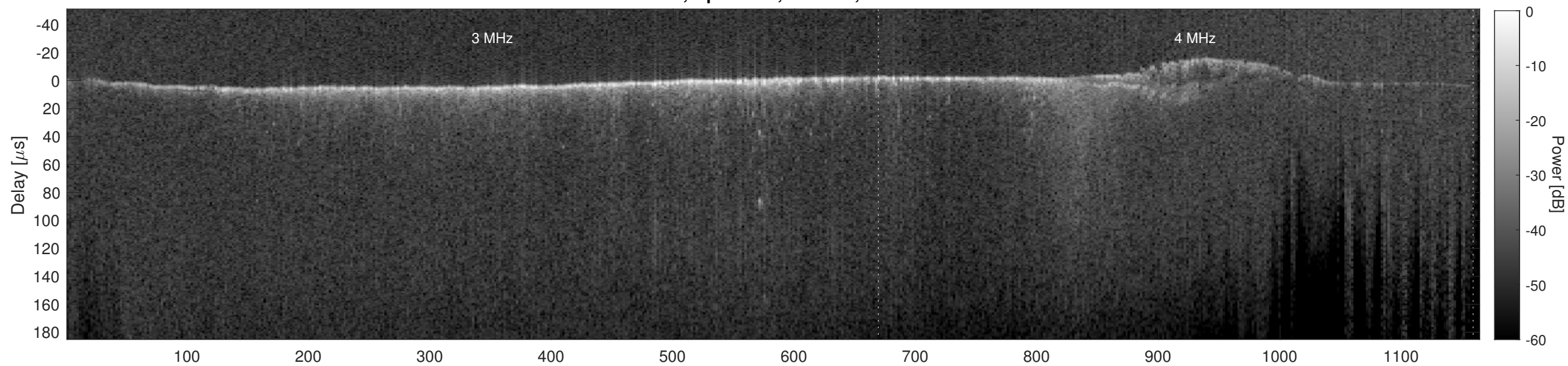
Orbit 7865, Cluttergram
