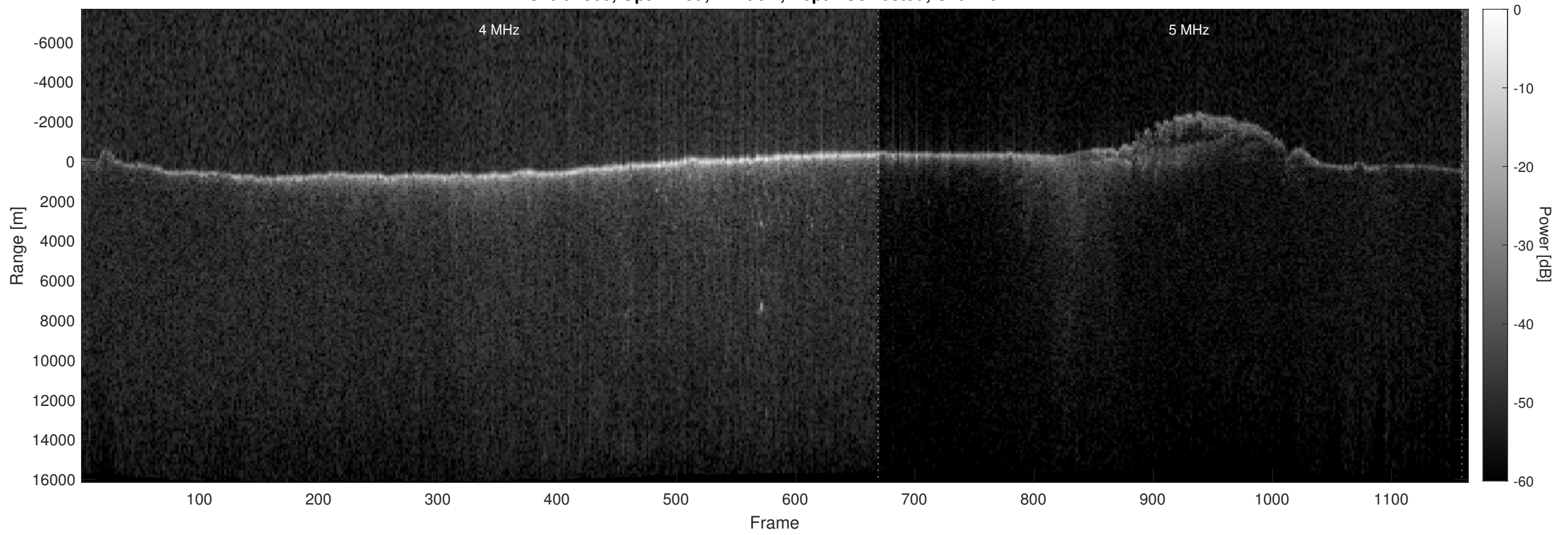
Orbit 7865, Optimized, Window, Depth-Corrected, Channel 2
