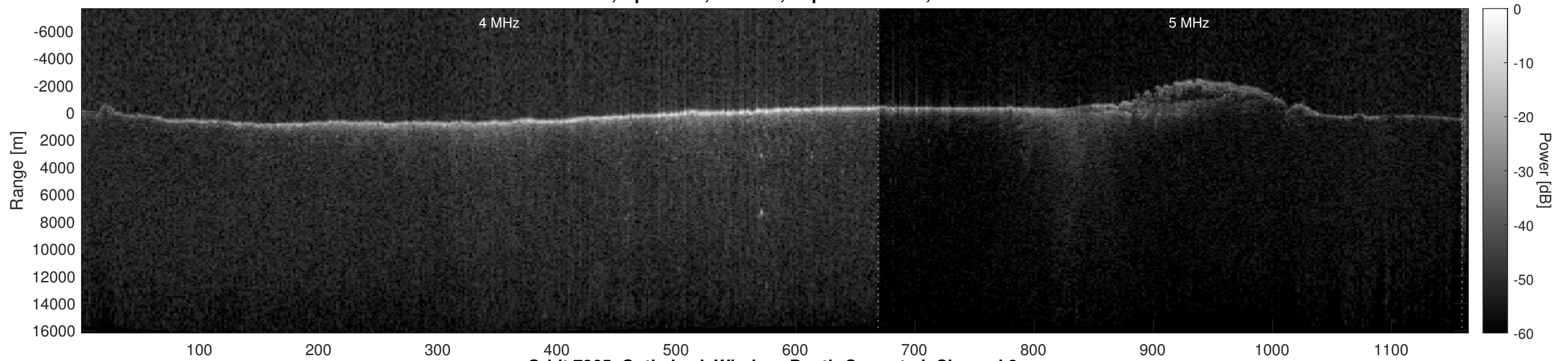
Orbit 7865, Optimized, Window, Depth-Corrected, Channel 2
