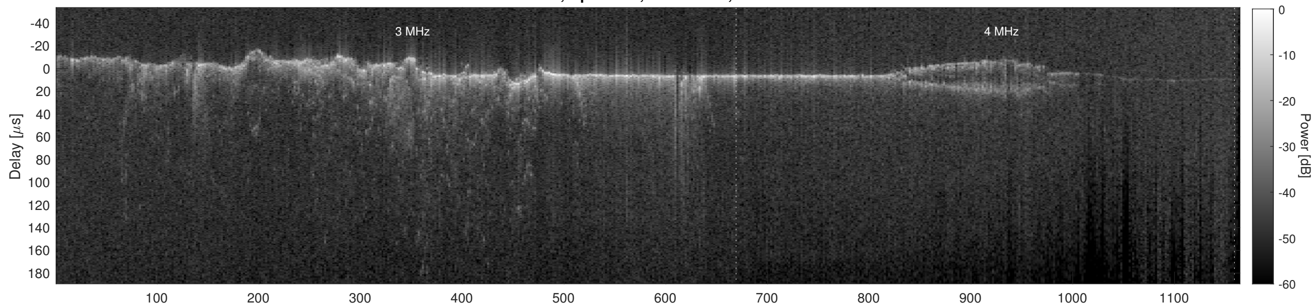
Orbit 7866, Cluttergram
