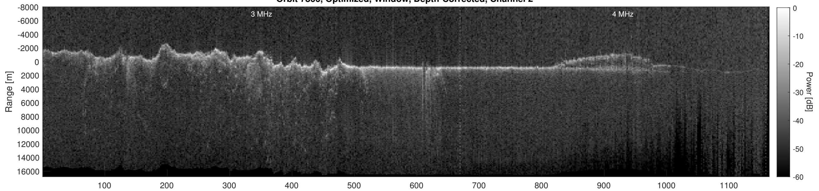
Orbit 7866, Depth-Corrected Cluttergram
