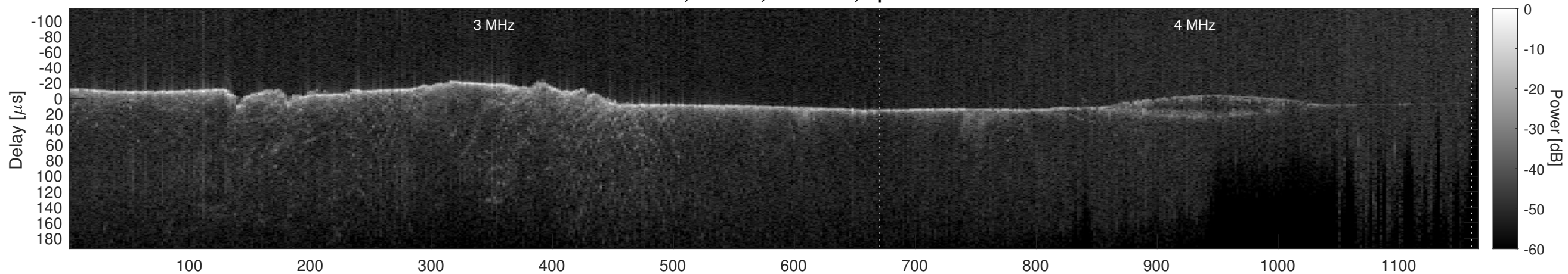
Orbit 7867, Cluttergram
