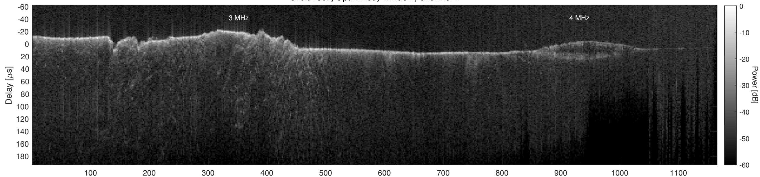
Orbit 7867, Cluttergram
