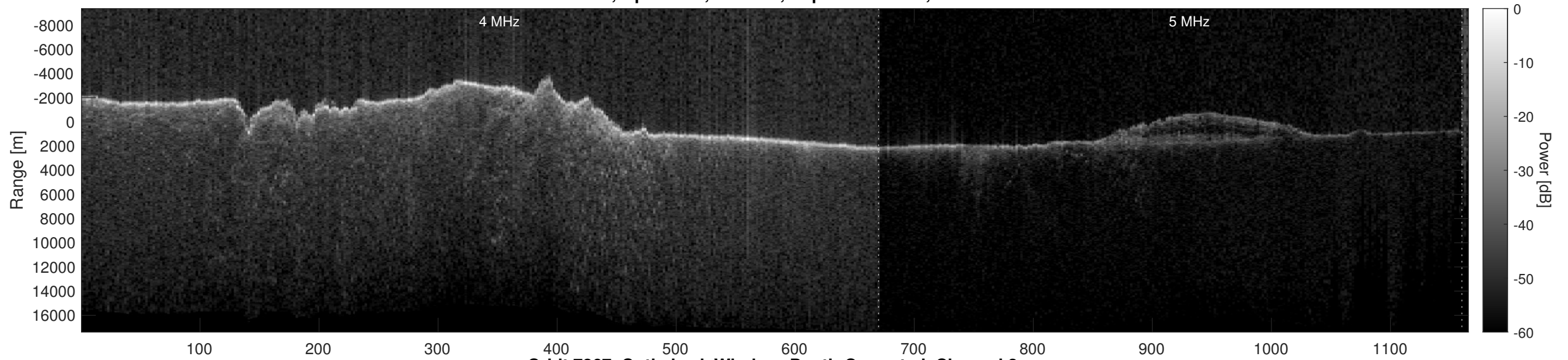
Orbit 7867, Optimized, Window, Depth-Corrected, Channel 2
