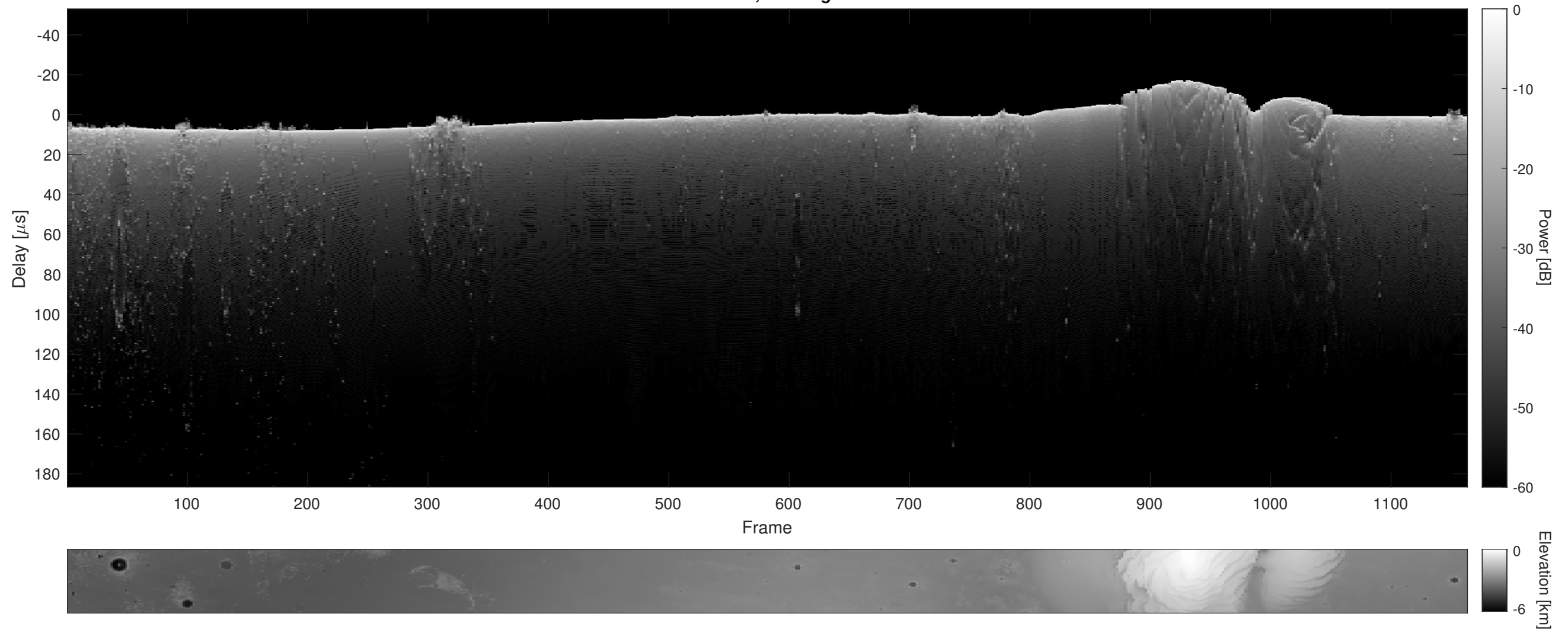
Orbit 7868, Cluttergram
