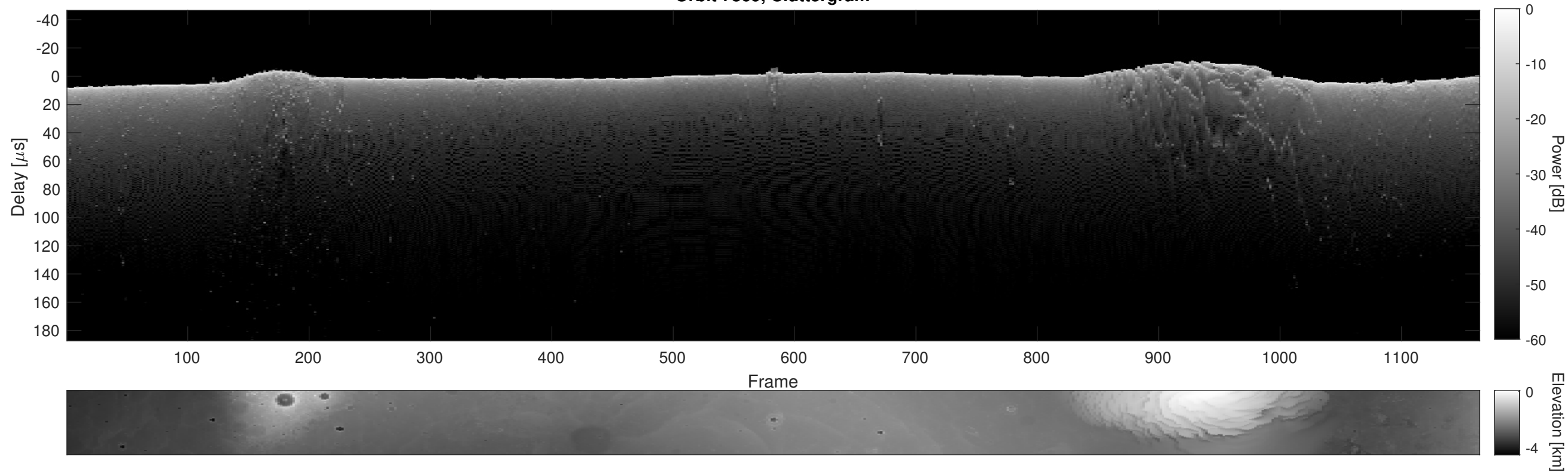
Orbit 7869, Cluttergram
