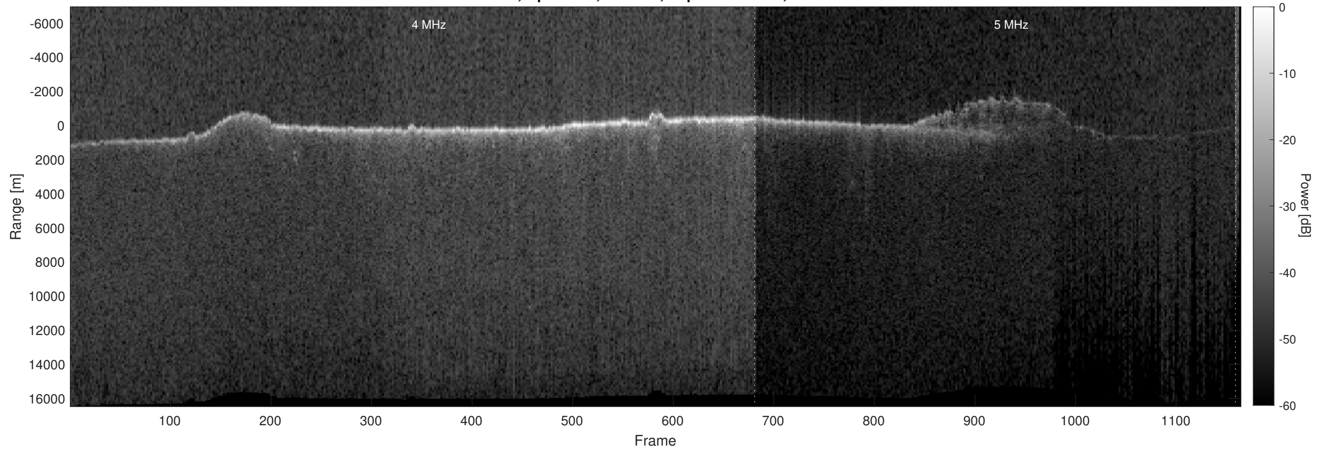
Orbit 7869, Optimized, Window, Depth-Corrected, Channel 2
