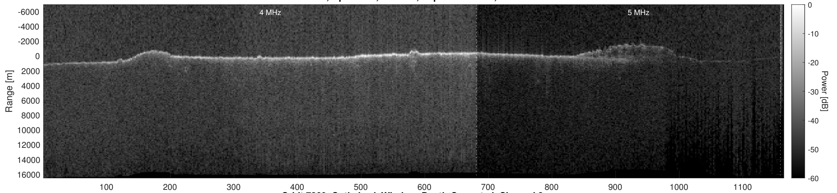
Orbit 7869, Optimized, Window, Depth-Corrected, Channel 2
