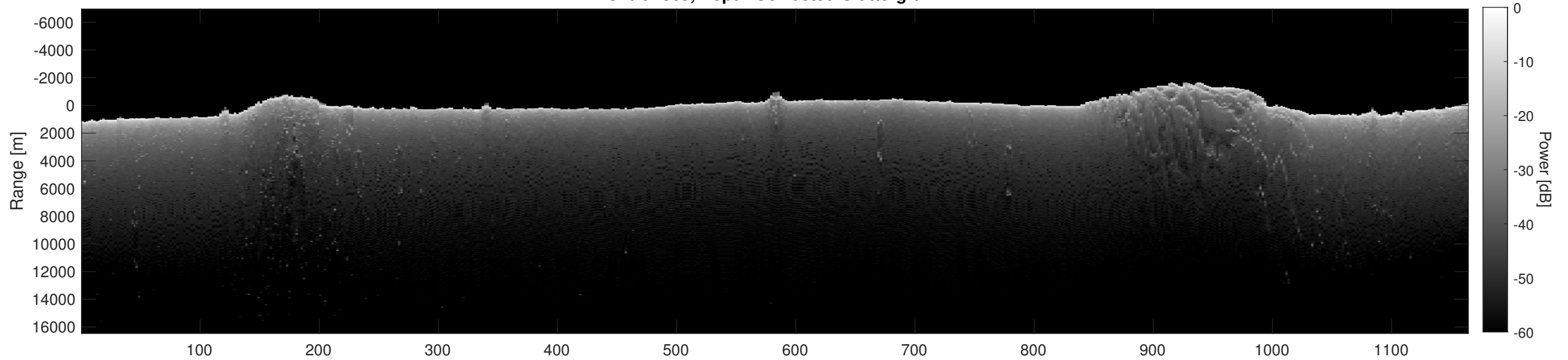
Orbit 7869, Depth-Corrected Cluttergram
