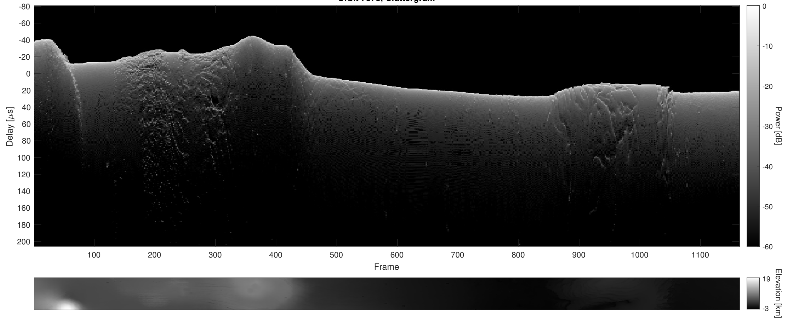
Orbit 7878, Cluttergram
