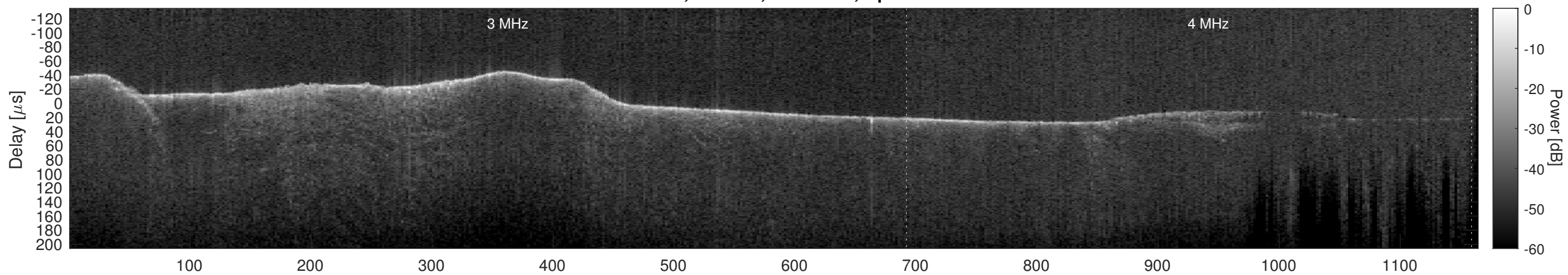
Orbit 7878, Cluttergram
