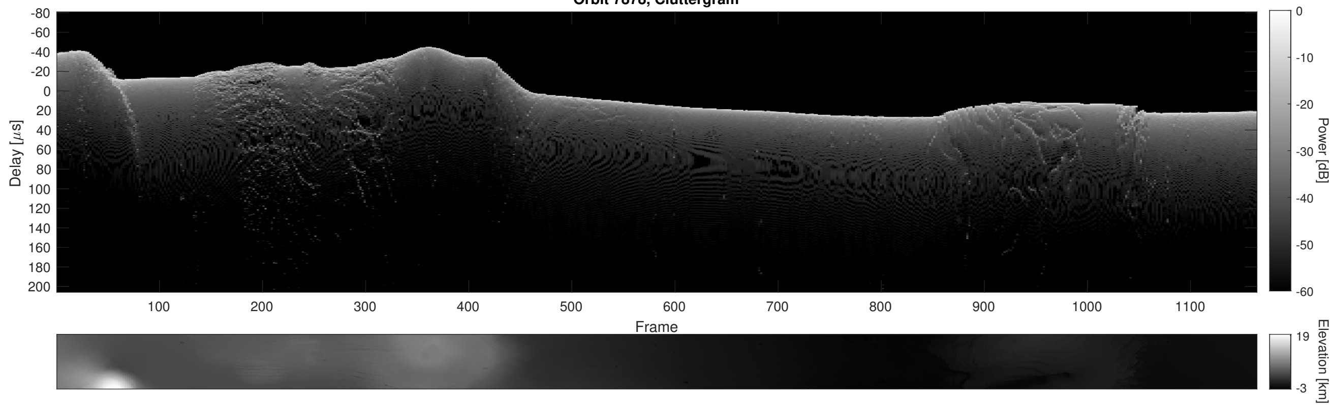
Orbit 7878, Cluttergram
