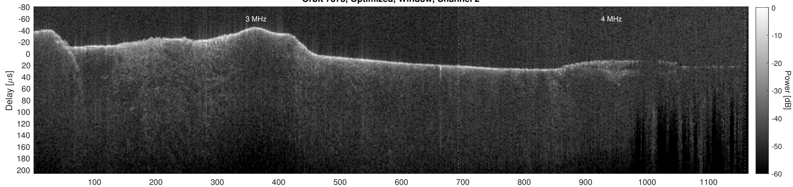
Orbit 7878, Cluttergram
