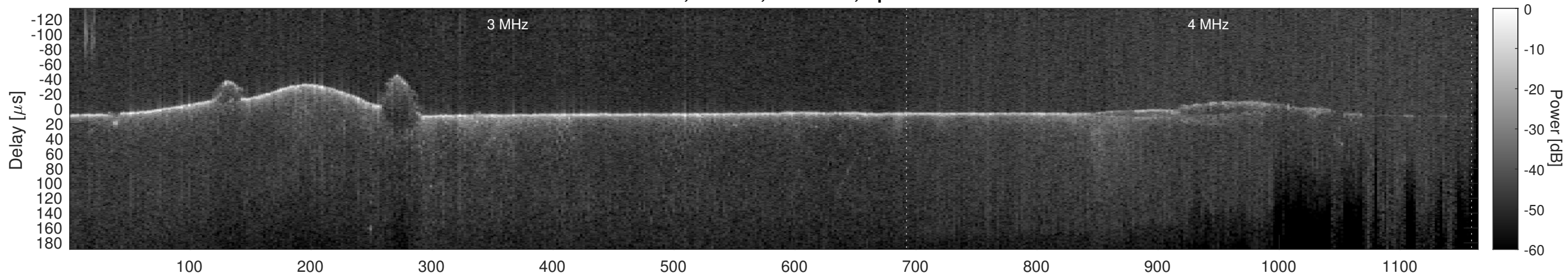
Orbit 7879, Cluttergram
