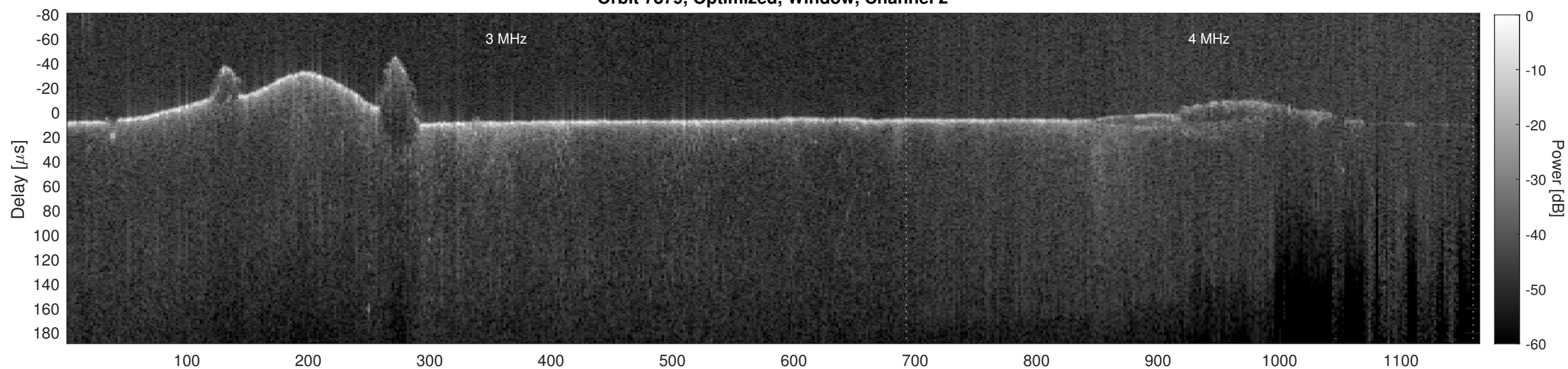
Orbit 7879, Cluttergram
