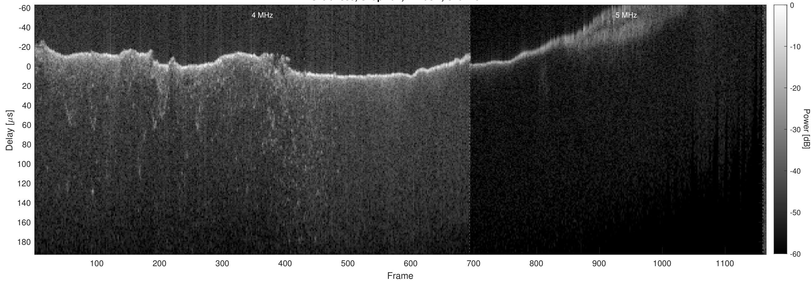
Orbit 7880, Chapman, Window, Channel 2
