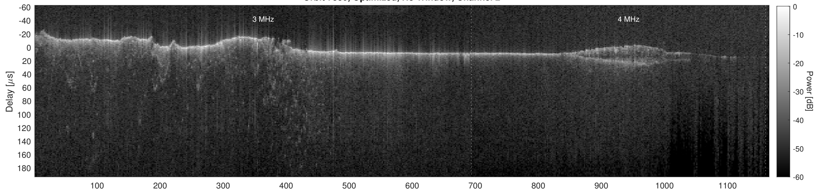
Orbit 7880, Cluttergram
