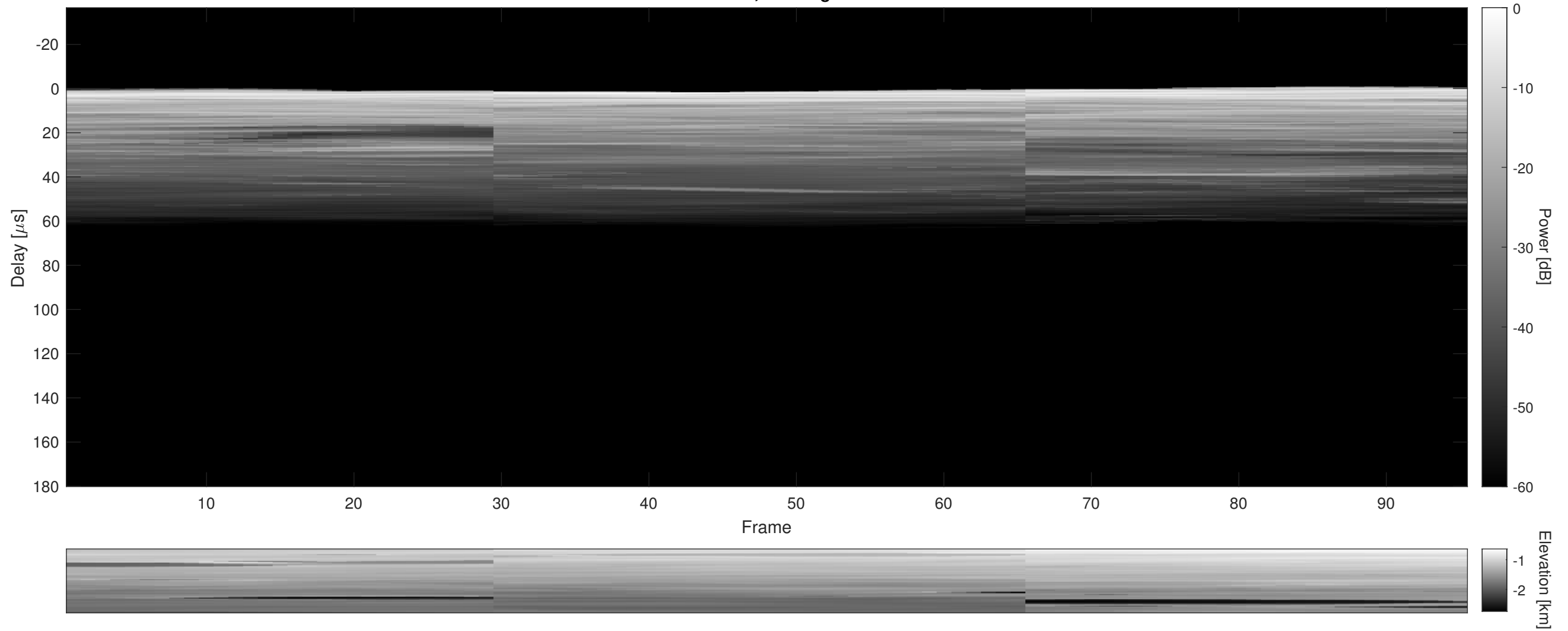
Orbit 7882, Cluttergram
