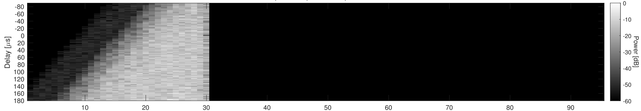
Orbit 7882, Window, Channel 2, Chapman
