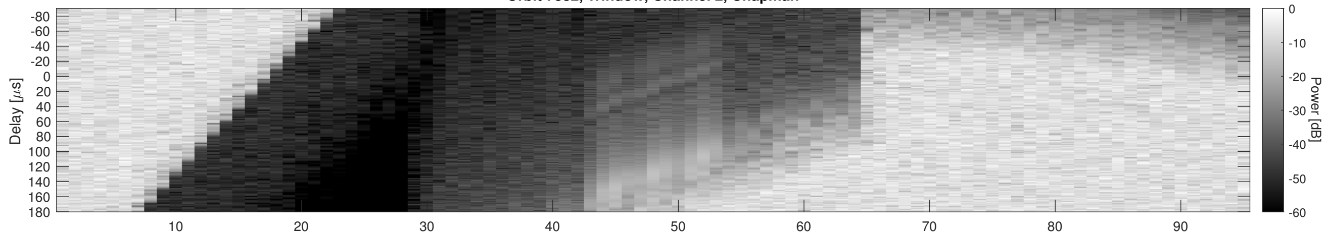
Orbit 7882, Window, Channel 2, Optimized
