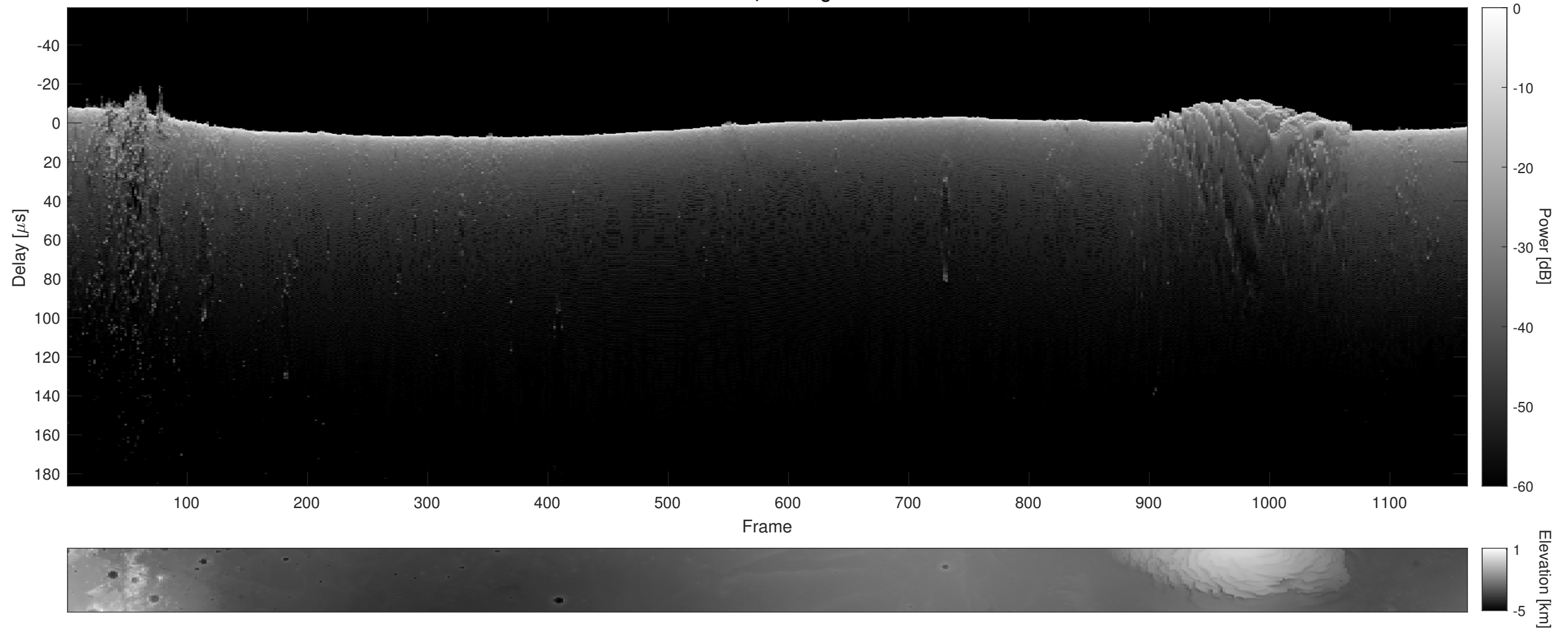
Orbit 7883, Cluttergram
