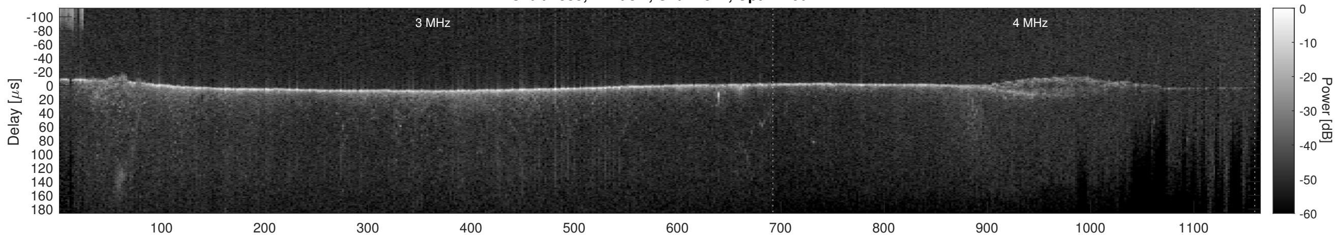
Orbit 7883, Cluttergram
