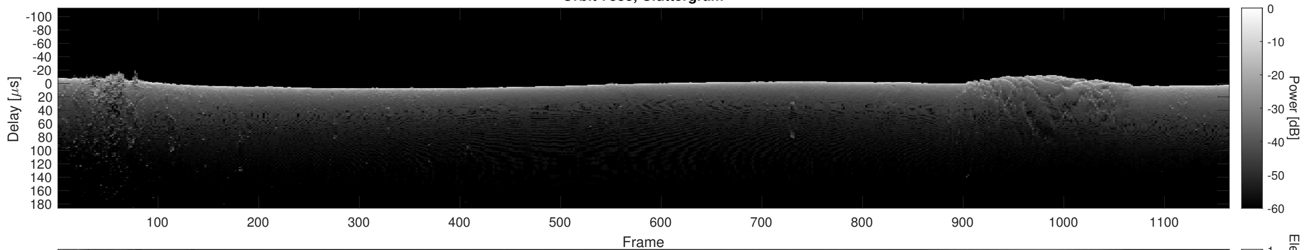
Orbit 7883, Cluttergram
