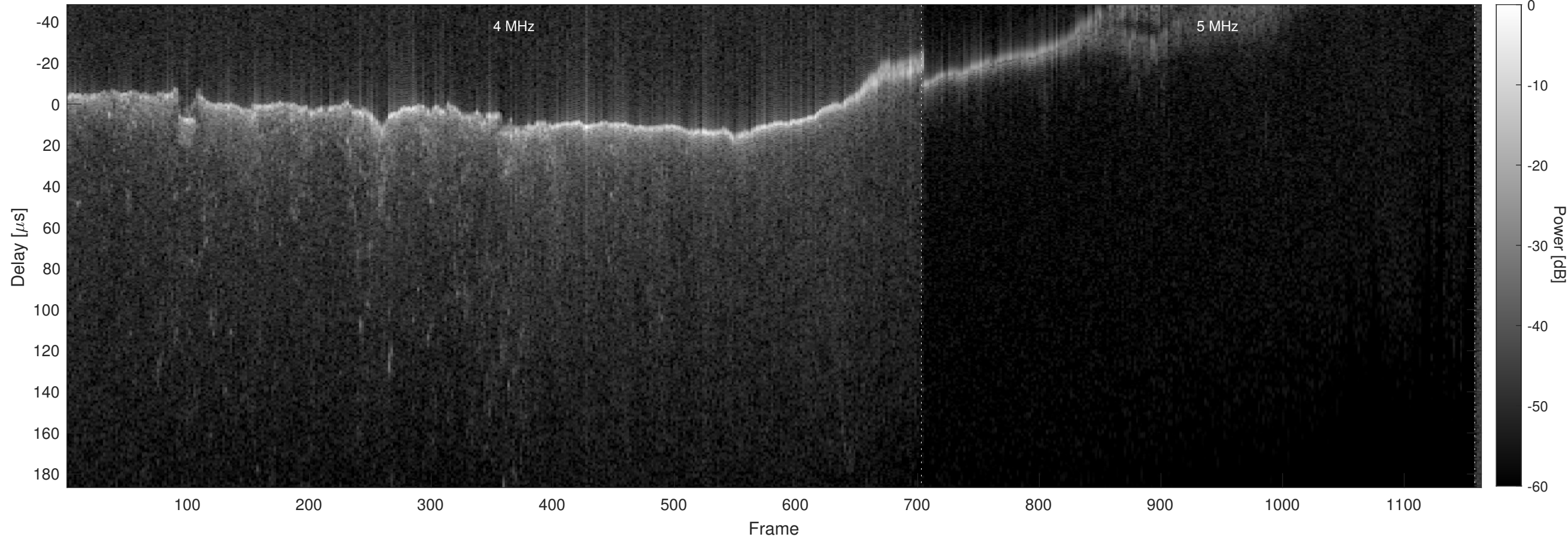
Orbit 7884, Chapman, No Window, Channel 2
