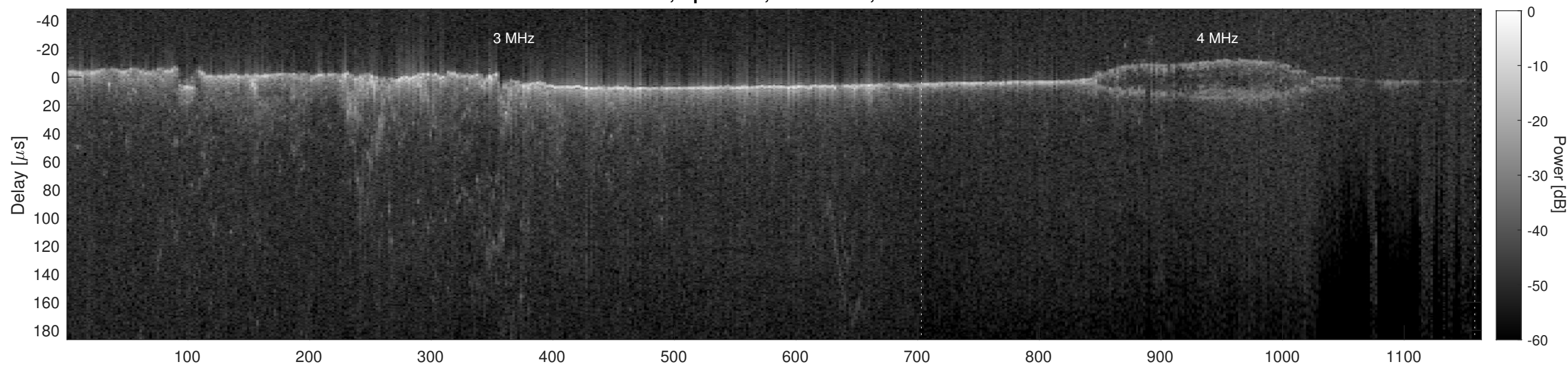
Orbit 7884, Cluttergram
