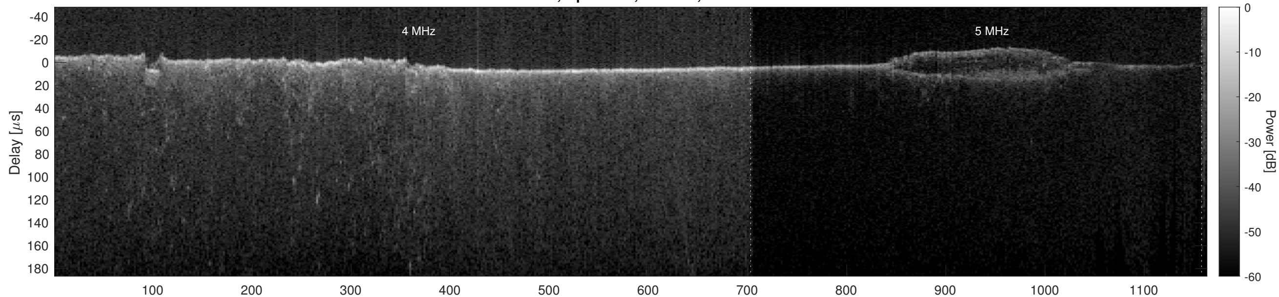
Orbit 7884, Optimized, Window, Channel 2
